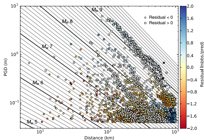
▲ Figure 4. PGD measurements with hypocentral distance colored by residual. Circles are negative residuals, and squares are positive residuals. Oblique lines are the predicted scaling values from the least-squares regression of the PGD measurements as a function of hypocentral distance. The color version of this figure is available only in the electronic edition.
