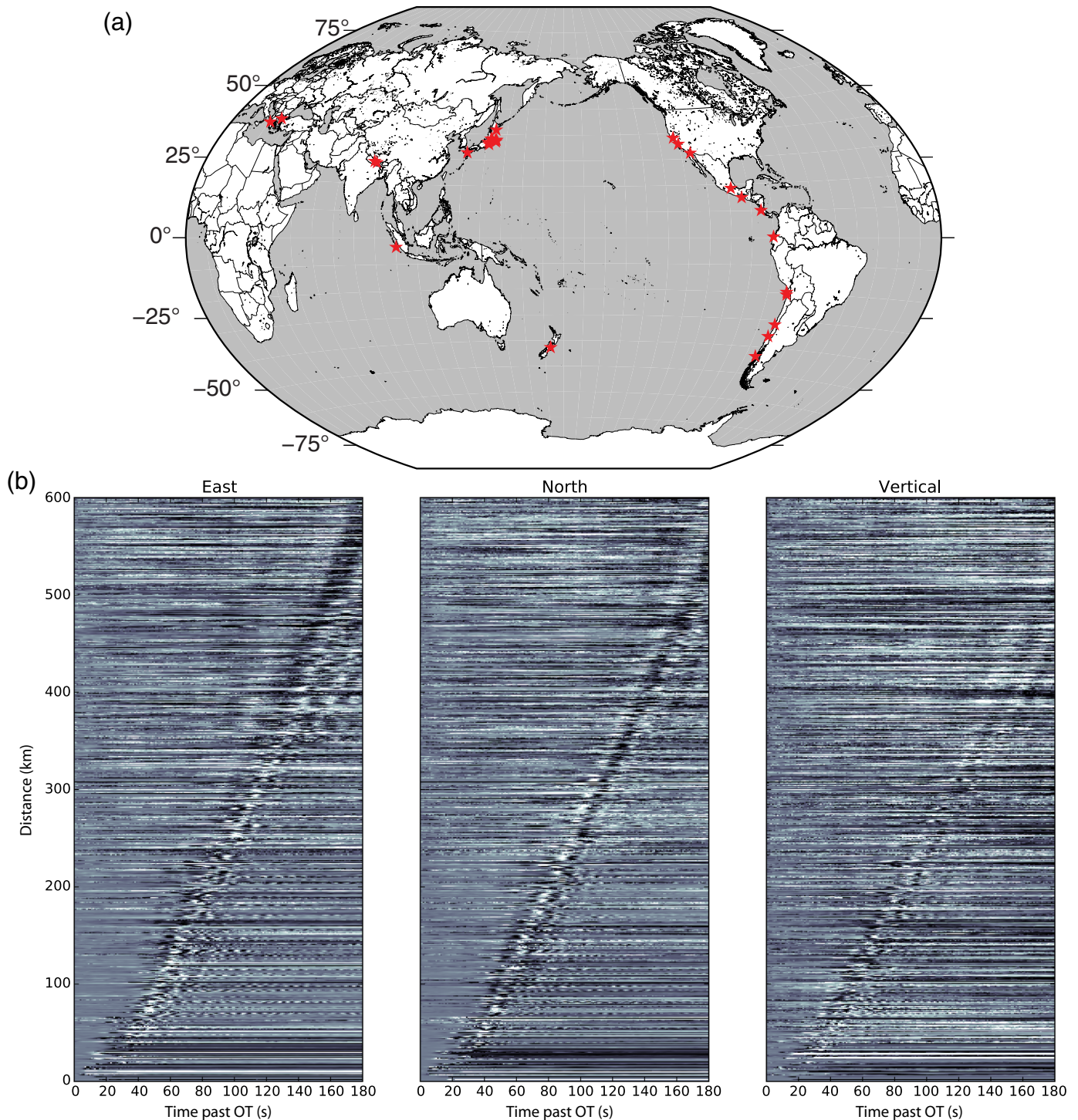
▲ Figure 1. (a) Map of 29 earthquakes and (b) three-component displacement waveforms within 600 km hypocentral distance for all 29 earthquakes. The color version of this figure is available only in the electronic edition.
