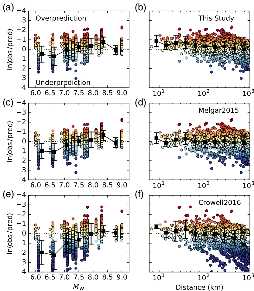
▲ Figure 5. Residuals plotted (a) as a function of earthquake magnitude and (b) as a function of hypocentral distance for PGD–magnitude scaling laws derived (top row) in this study, (middle row) by Melgar et al. (2015), and (bottom row) by Crowell et al. (2016). Medians (black squares) with one standard deviation error bars are shown. The color version of this figure is available only in the electronic edition.
