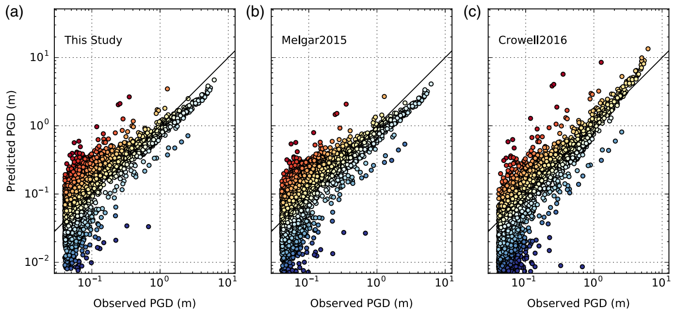
▲ Figure 3. Predicted versus observed PGD for the coefficients found in (a) this study, (b) Melgar et al. (2015) , and (c) Crowell et al. (2016) . The color version of this figure is available only in the electronic edition.
