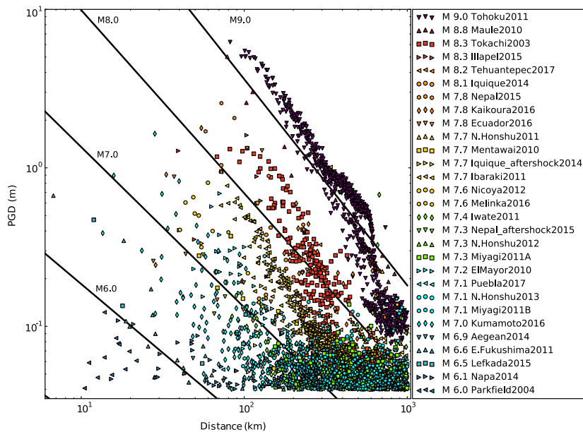
▲ Figure 2. Peak ground displacement (PGD) measurements with hypocentral distance. Oblique lines are the predicted scaling values from the least-squares regression of the PGD measurements as a function of hypocentral distance. The color version of this figure is available only in the electronic edition.
