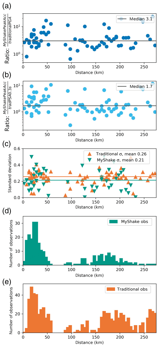
Figure 10. (a) The ratio of MyShake peak acceleration versus traditional station peak ground acceleration (PGA), as binned over 5 km increments for the five sample events. (b) The ratio of MyShake peak acceleration versus 0.3 s pseudospectral acceleration (PSA) from traditional stations. (c) The standard deviation of the log10 of MyShake and traditional station peak acceleration measurements. (d) The number of MyShake observations for all events binned by epicentral distance. (e) The number of traditional station observations for all events binned by epicentral distance.
